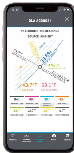
Psychrometric Chart
